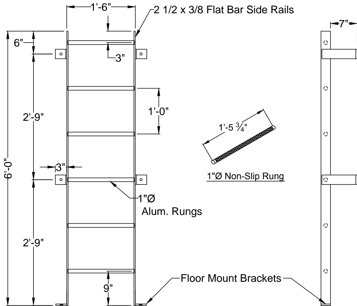
Front Elevation
